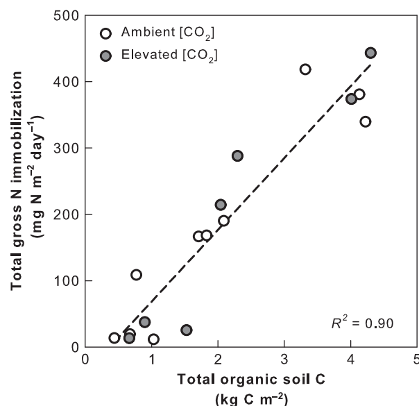
Fig. 2 Positive relationship between soil organic C content and total gross N immobilization [gross N mineralization – net \text{NH}_4^+ + \text{NO}_3^- mineralization]. Data points are treatment rings at each soil depth; data were omitted if total N immobilization was < 0 (3 points total, 30–60 cm soil depth). While there were greater root C inputs over 10 years under elevated carbon dioxide concentrations [\text{CO}_2] (filled circles), there was no difference in the relationship between soil C content and total gross N immobilization between \text{CO}_2 treatments. Total gross N immobilization = -39.7 + 108.2 \times \text{soil C content} ( R^2 = 0.90 , P < 0.0001 ).
