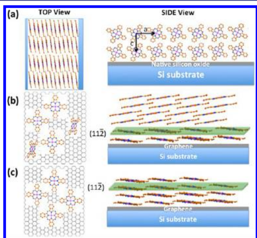
Figure 4. Schematic representations of the possible molecular packing orientations of the CuPc film grown on (a) silicon, (b) graphene at room temperature, and (c) graphene at 130 °C.
