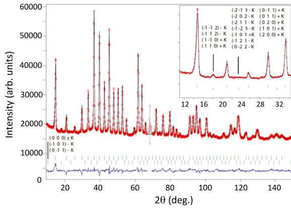
Figure 3. Diffractogram measured at 1.8 K. The solid curve is the best fit of the data employing the ‘quantum model’ for the magnetic phase. The first row of green lines indicates the positions of the reflections indexed in Im\bar{3}m with a = 13.291(2) Å. The second line indicates the magnetic phase with a PV K = (0, 0, 1) , or its equivalents, in the space group Im\bar{3}m . The inset enlarges the low-angle portion of the diffractogram, where the small magnetic peak around 2\theta = 18.1^\circ can be clearly observed. The (h, k, l) indices of three possible magnetic peaks at 2\theta = 10.4^\circ , 18.1^\circ and 23.4^\circ are indicated.
