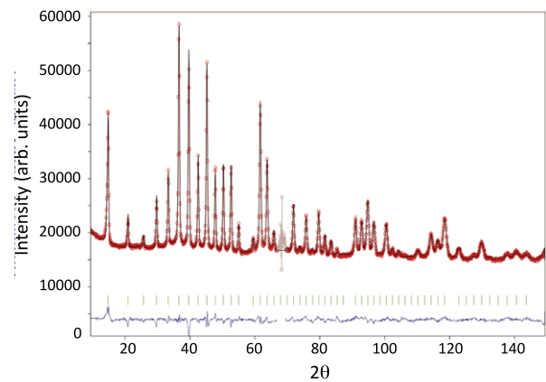
Figure 2. Diffraction pattern measured at 50 K. The solid curve is the best fit of the data employing the Rietveld method. The bottom blue curve is the difference between observed and calculated intensities. The green lines indicate the positions of the reflections indexed in Im\bar{3}m with a = 13.3028(2) Å.
