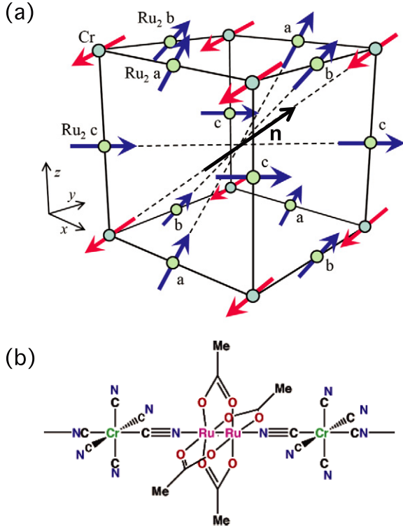
Figure 1. (a) The predicted ground state of a single sublattice of \text{Cr}(\text{Ru}_2)_3 for infinite anisotropy and classical spins. The net sublattice spin points along \mathbf{n} = (1, 1, 1)/\sqrt{3} or one of the 8 different cubic diagonals. (b) A sketch of the \text{Ru}_2 complex with surrounding Me ‘paddlewheel’. Reproduced with permission from [5]. Copyright 2009 American Physical Society.
