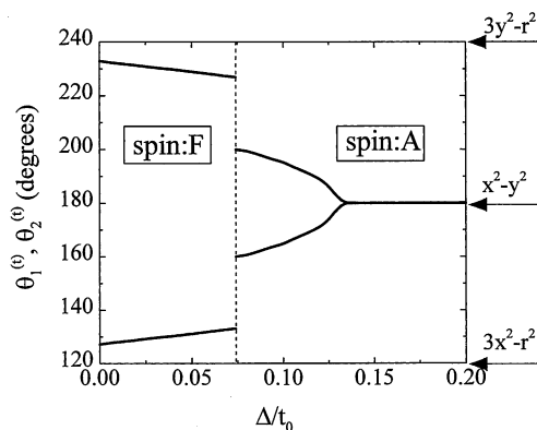
Fig. 2. The angles ( \theta_1^{(t)}, \theta_2^{(t)} ) in the orbital space as a function of \Delta . The angles 120^\circ , 180^\circ and 240^\circ correspond to the d_{3x^2-r^2} , d_{x^2-y^2} and d_{3y^2-r^2} orbitals, respectively.
