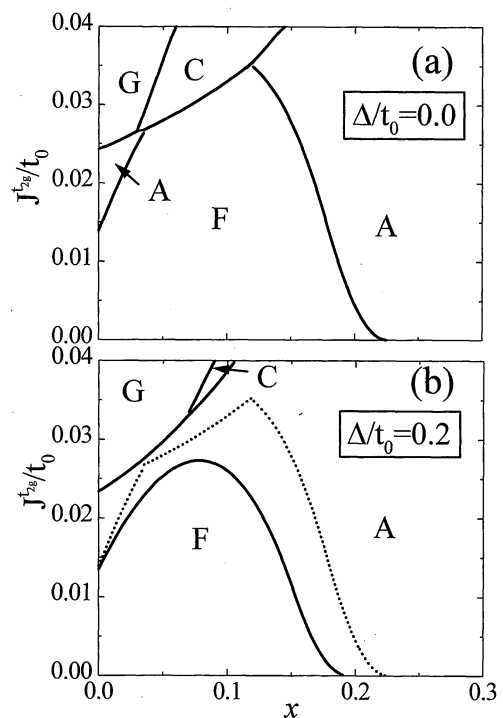
Fig. 1. The spin phase diagram with and without the energy level difference \Delta between two e_g orbitals. The dotted line in Fig. 1(b) shows the phase boundary between the spin:F phase and the other spin phases for \Delta = 0.0 case.
