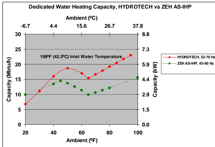
Figure 6: Comparison of dedicated water heating capacities for 2-ton (7 kW) HydroTech vs. ZEH AS-IHP
