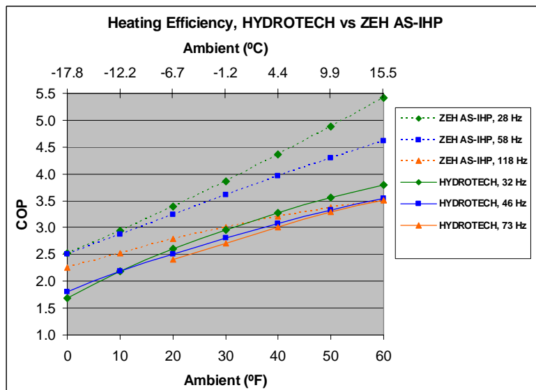
Figure 5: Comparison of space heating efficiencies for ZEH AS-IHP vs. HydroTech
