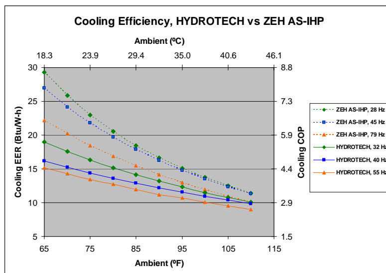
Figure 3: Comparison of space cooling efficiencies for ZEH AS-IHP vs. HydroTech
