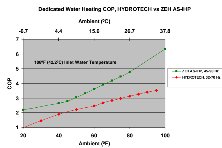
Figure 7: Comparison of dedicated water heating COPs for ZEH AS-IHP vs. HydroTech
