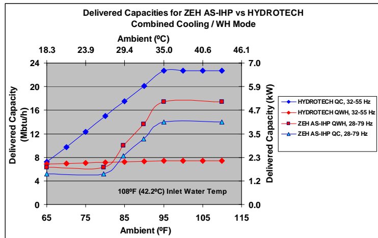
Figure 8: Space cooling and water heating capacities vs. ambient, dual mode
