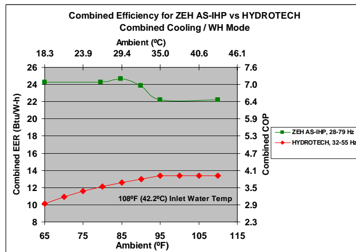
Figure 9: Combined efficiency for total cooling / water heating outputs vs. ambient, dual mode
