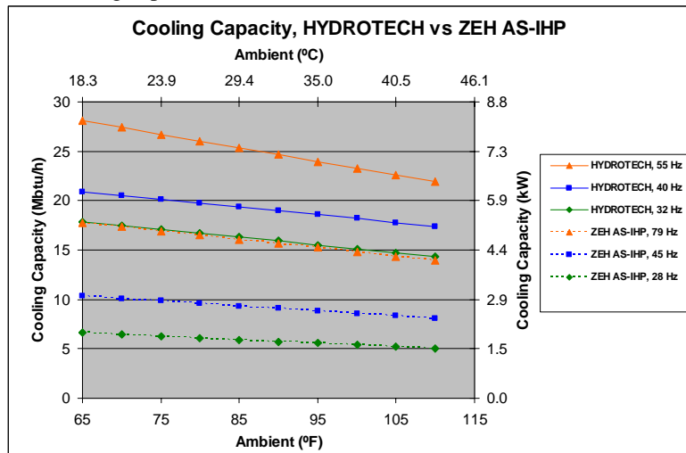
Figure 2: Comparison of space cooling capacities for 2-ton (7 kW) HydroTech vs. 1.25-ton (4.4 kW) ZEH AS-IHP
