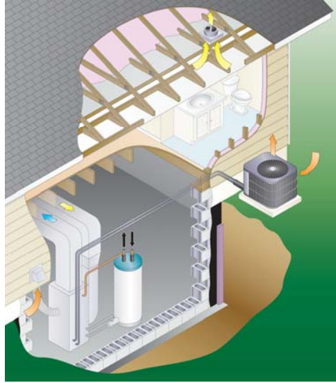
Figure 1: Conceptual installation of a residential air-source integrated heat pump.
