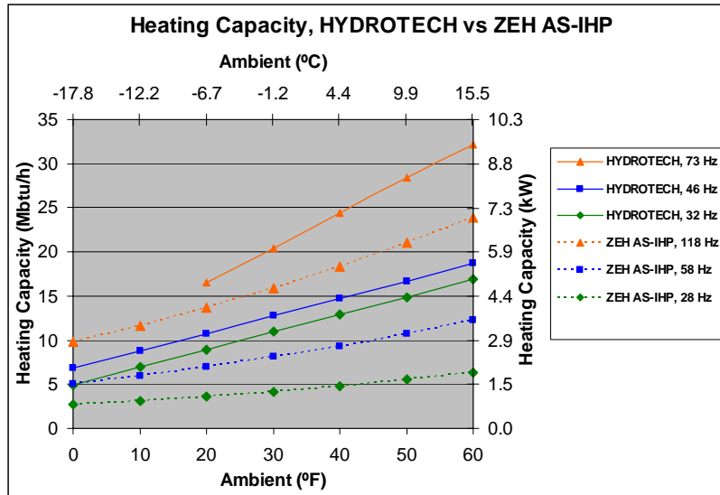
Figure 4: Comparison of space heating capacities for 2-ton (7 kW) HydroTech vs. ZEH AS-IHP
