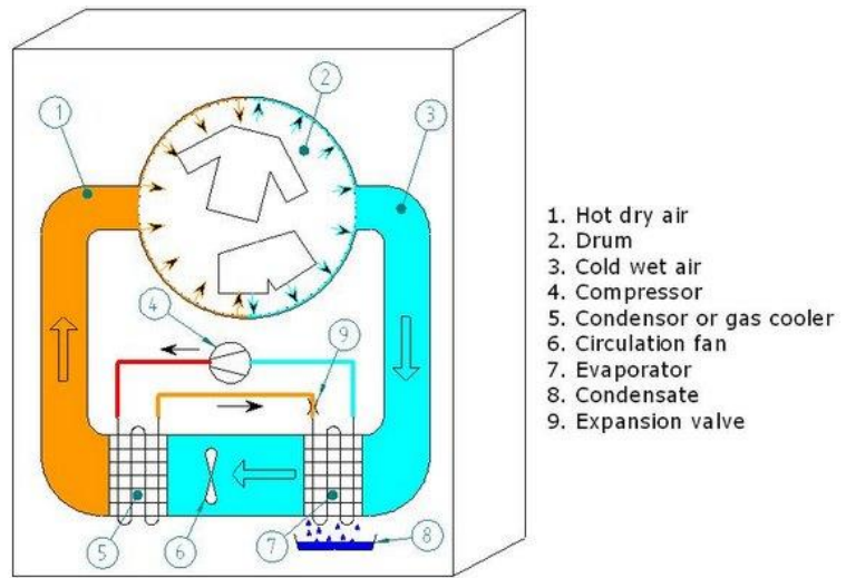
Figure 2: Schematics of a heat pump clothes dryer
