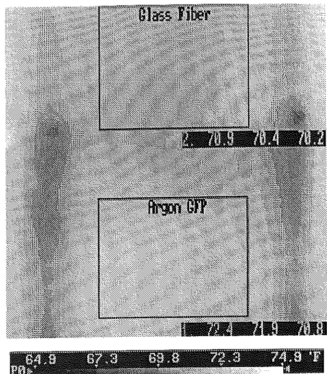
Figure 3 Infrared image of the warm-side surface of a stud wall cavity test section. The upper portion of the cavity is insulated with R-11 h·ft 2 ·°F/Btu (1.9 m 2 ·K/W) glass fiber insulation and the lower portion with a prototype argon GFP. The wall section is constructed with 0.75-in. (0.019-m) plywood, 0.625-in. (0.016-m) drywall, and standard 16 in. (0.41 m) on center 2-by-4 studs. The back of this assembly faces a cold chamber at -19.9°F (-28.8°C); ambient temperature is 74.0°F (23.3°C). The warm-side surface temperature of the fiber-glass-insulated section averages 70.4°F (21.4°C), while the argon GFP-insulated section averages 71.9°F (22.1°C). A corresponding temperature gray scale is shown at the bottom of the figure. Since surface temperatures correspond to heat loss rates, the argon GFP's higher warm-side temperature implies a lower heat loss rate.
