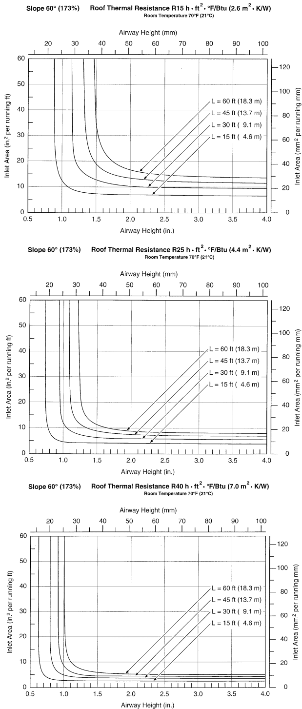
Figure 10 Airway heights and inlet areas for cathedral ceilings with a slope of 60°.
