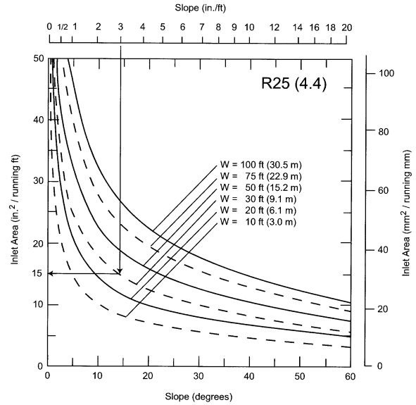
Figure 4 Net free open area of inlets for attics with R25 (in SI units, R4.4) insulation.
