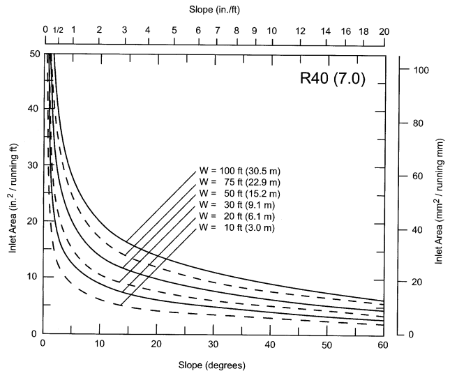
Figure 5 Net free open area of inlets for attics with R40 (in SI units, R7.0) insulation.
