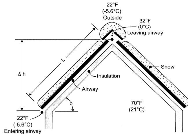
Figure 6 A typical ventilated cathedral ceiling.
