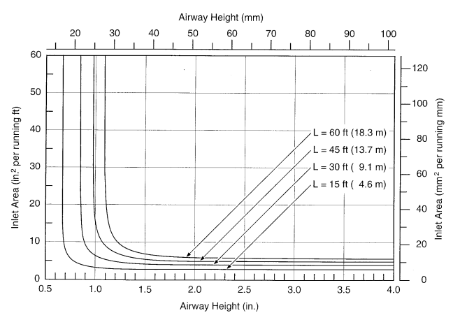
Slope 45° (100%) Roof Thermal Resistance R40 h · ft 2 · °F/Btu (7.0 m 2 · K/W) Room Temperature 70°F (21°C)
