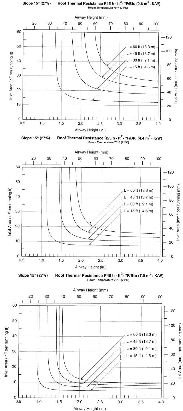
Figure 7 Airway heights and inlet areas for cathedral ceilings with a slope of 15°.
