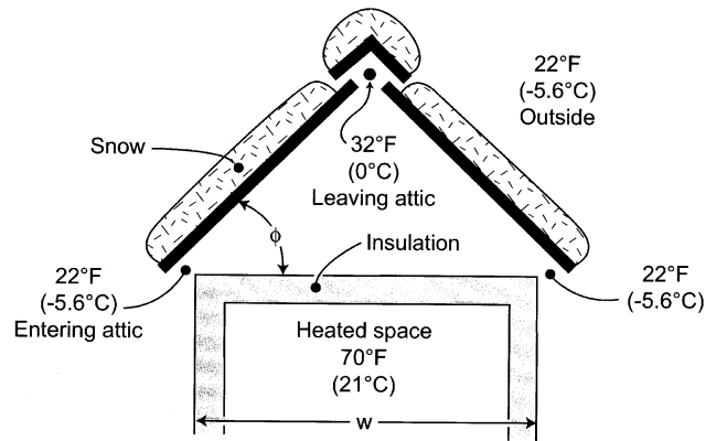
Figure 2 A typical ventilated attic at the “design” condition.
