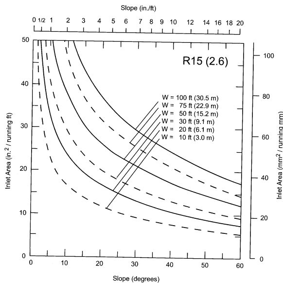
Figure 3 Net free open area of inlets for attics with R15 (in SI units, R2.6) insulation.
