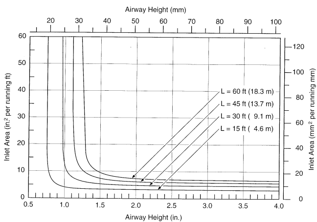
Slope 30° (58%) Roof Thermal Resistance R40 h · ft 2 · °F/Btu (7.0 m 2 · K/W) Room Temperature 70°F (21°C)
