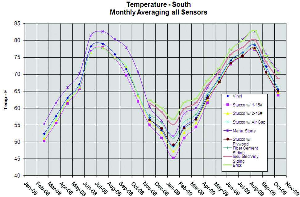
Figure 6 Wall cavity temperature: south.
